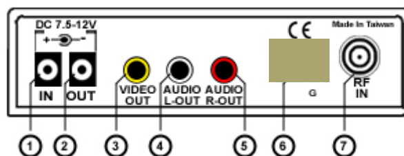
Rear Panel
